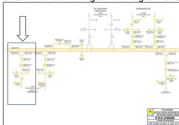
Gambar 2 Single Line Diagram Gardu Induk Jatibarang 70kV
